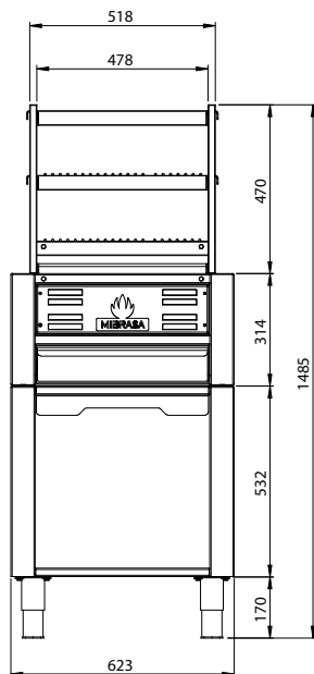
VISTA FRONTAL
