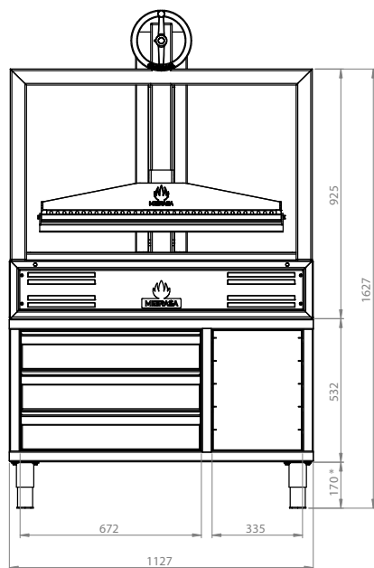
VISTA FRONTAL
