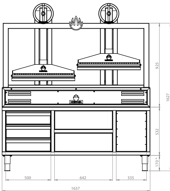
VISTA FRONTAL
