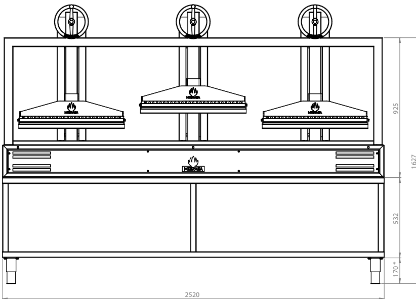
VISTA FRONTAL
